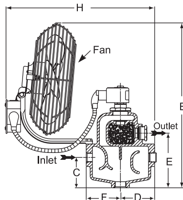
Figure 63-1. FSA humidifiers
