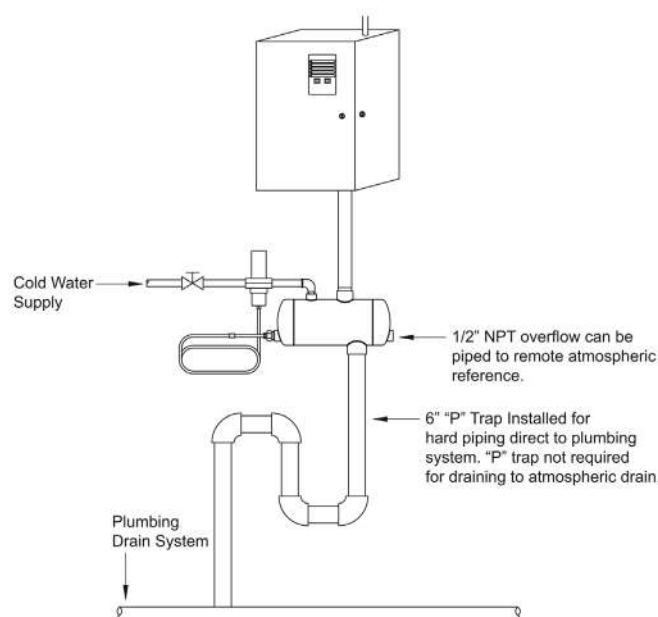
Figure 149-2. Typical Installation
