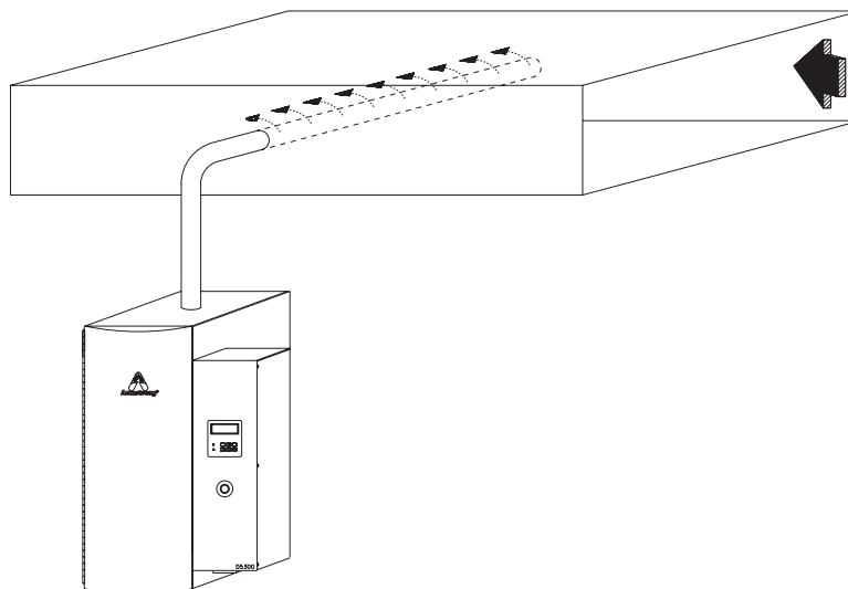
Figure 142-2. HC-6100 or 6300 Duct Type Distribution
