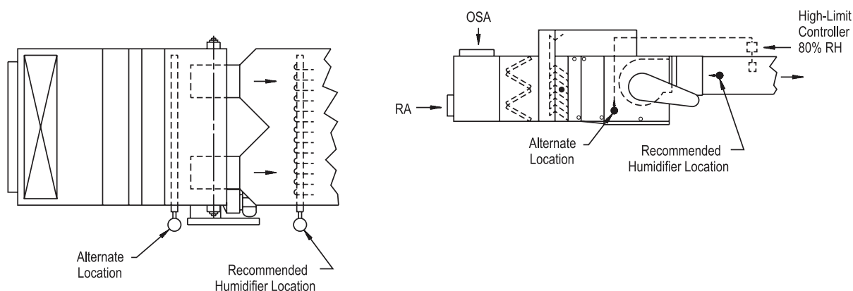
Figure 35-2. Vertical Discharge
