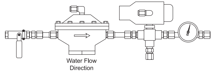
Figure 163-2. Water Valves
