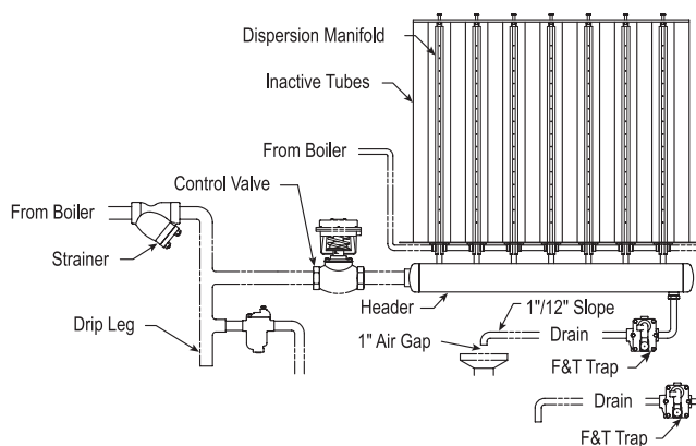
Figure 27-4. Steam Panel System
