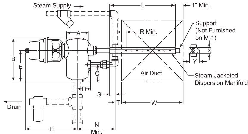
Figure 72-1. Dimensions
