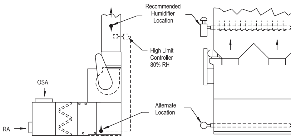
Figure 35-2. Vertical Discharge
