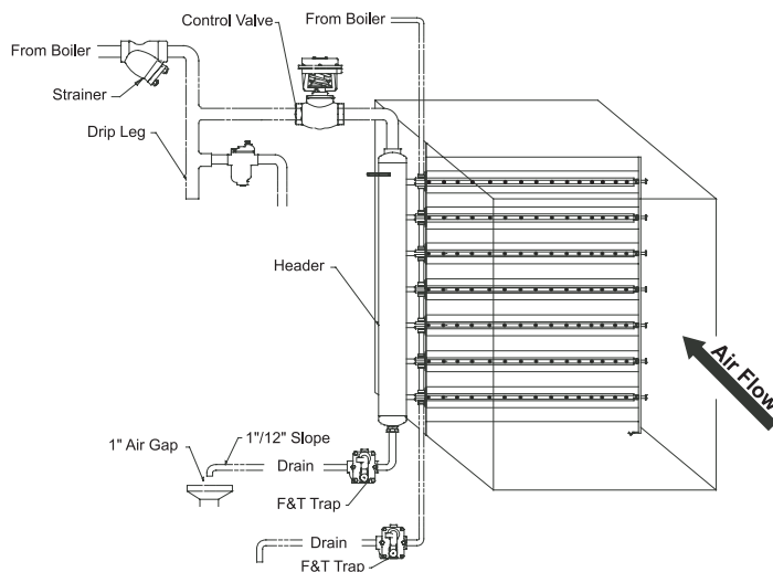
Figure 80-2. HumidiPackPlus
