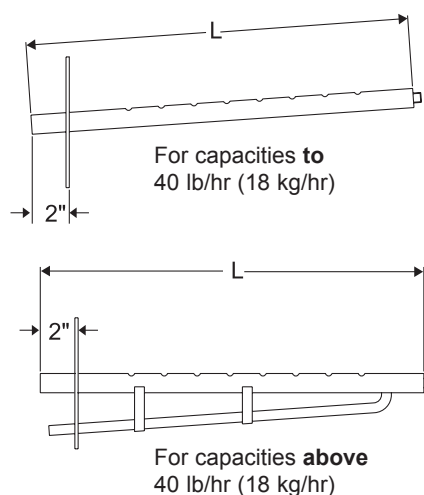
Figure 152-1. Dispersion Tube
