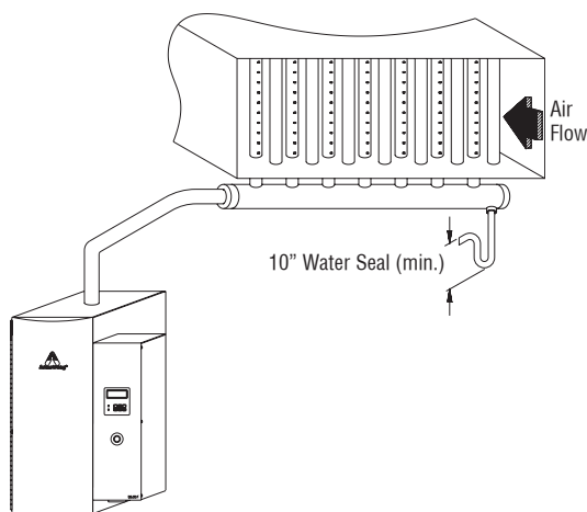
Figure 122-4. HC-6100 or HC-6300 HumidiClean Piped to HumidiPack
