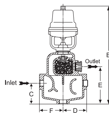
Figure 65-2. AM humidifiers
