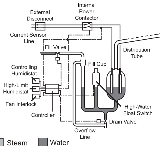
Figure 131-3. No demand. Contactor opens. No steam output.
