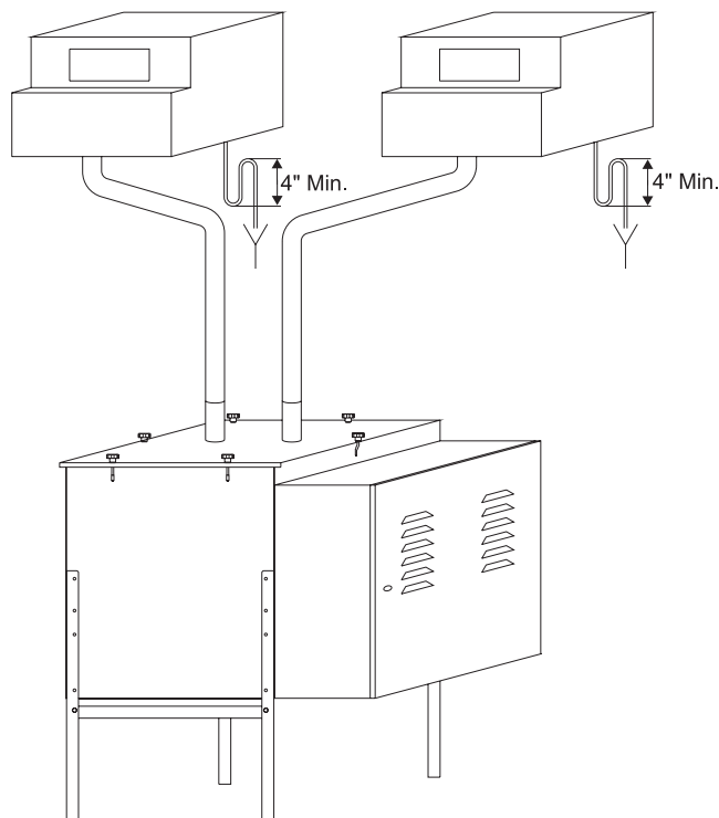
Figure 113-4 Duct Mounted Below Humidifier (Model GFH-150 shown)
