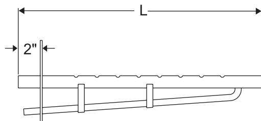
Figure 110-1. Armstrong DL type dispersion tube. Minimum of two required. See Table 118-1 above.
