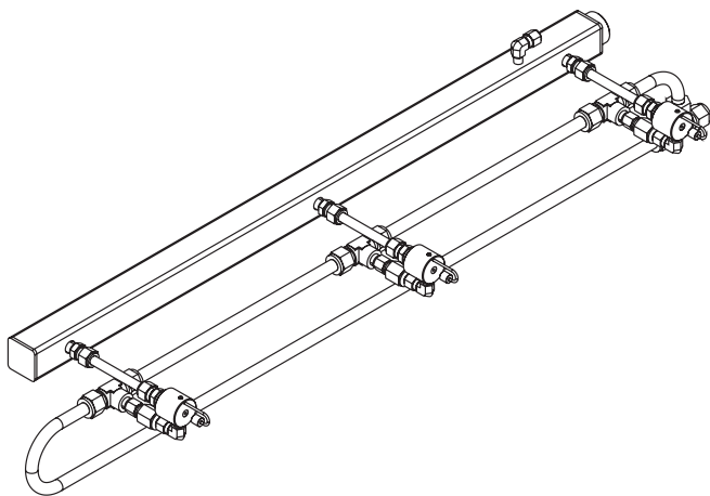
Figure 162-2. Area Discharge
