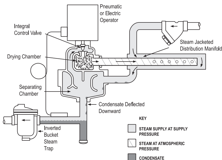
Figure 20-3. Steam Separator Type Humidifier
