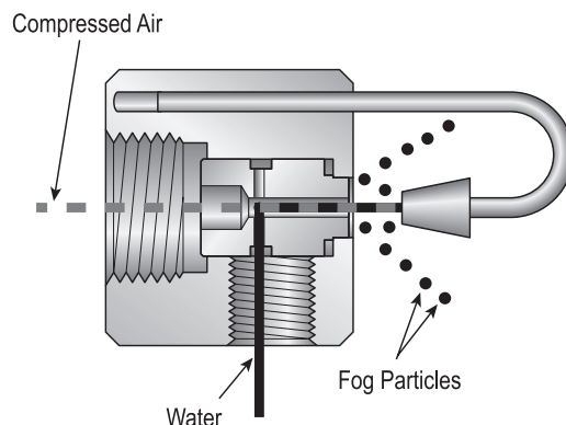
Figure 153-2. Fogger Head
