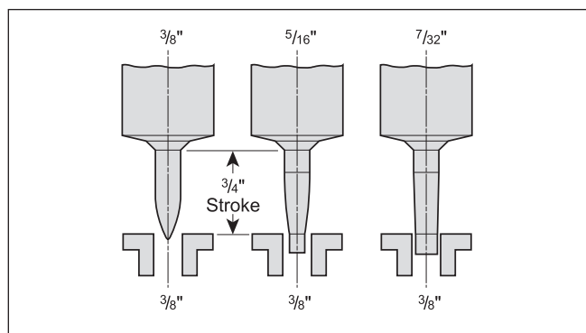
Figure 21-1. Parabolic Plug Metering Valve
