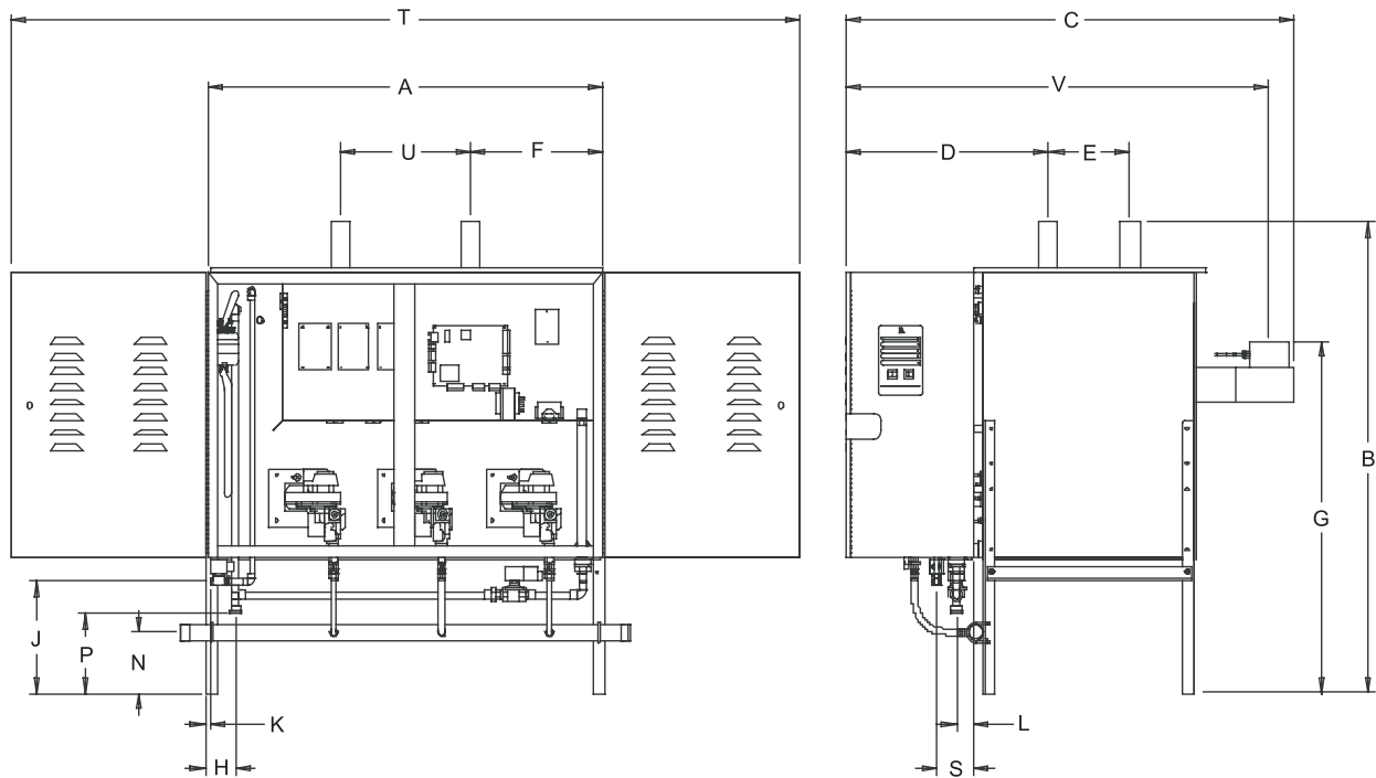
Figure 109-2. GFH-450 Dimensions
