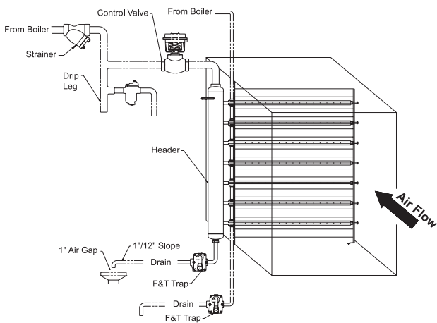
Figure 139-2. HumidiPackPlus
