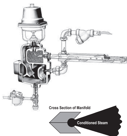
Figure 16-1. Separator Type
