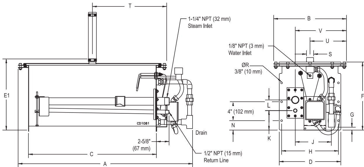
Figure 102-1. Model CS-11
