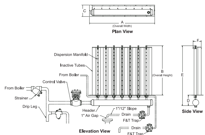
Figure 89-2. Vertical HumidiPackPlus
